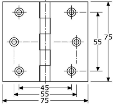
#42.578 - 75 mm x 75 mm x 2.5 mm; medium duty, for cabin doors 316 stainless steel. For screws 4.5/5 mm
