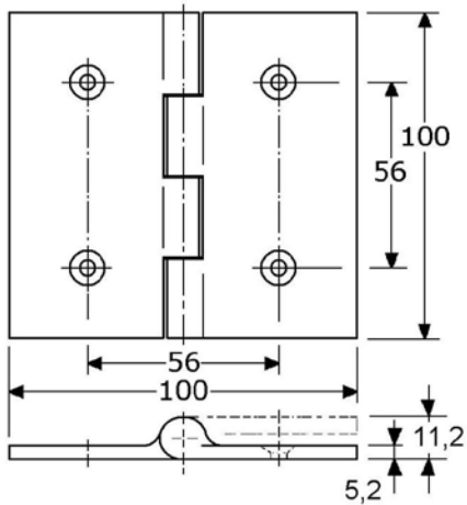
#42. 287 - 100 mm x 100 mm x 5.2 mm; heavy duty, for cabin and weather doors 316 stainless steel. For countersunk screws 4.5/5 mm
