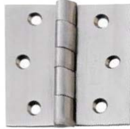
#42.578 - 75 mm x 75 mm x 2.5 mm; medium duty, for cabin doors 316 stainless steel. For screws 4.5/5 mm
