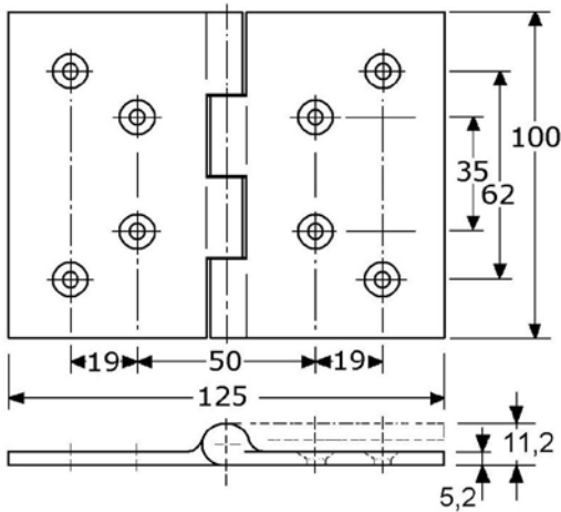
#42.262 - 100 mm x 125 mm x 5.2 mm; heavy duty, for cabin and weather doors 316 stainless steel. For countersunk screws 4.5/5 mm
